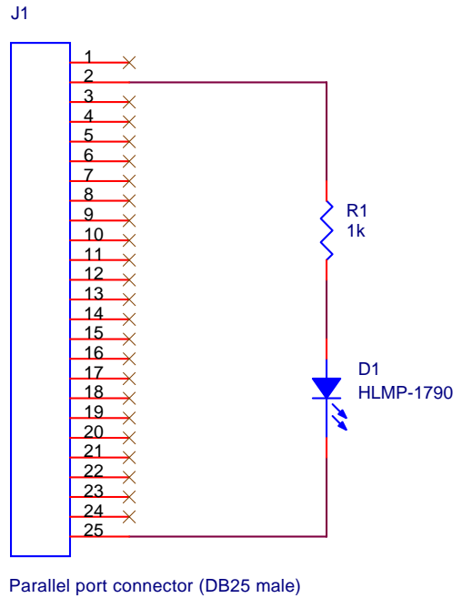
Parallel port connector (DB25 male)
